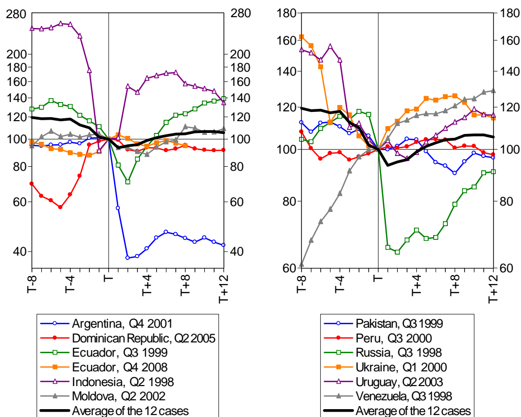
Figure A.1: Quarterly real effective exchange rate developments before and after twelve public debt defaults or restructurings during the past 15 years (quarter of restructuring = 100)
