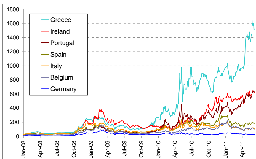
Figure 3: Credit default swap (CDS) spread on 5-year government bonds, 2 Jan 2008 – 6 June 2011, in basis points
