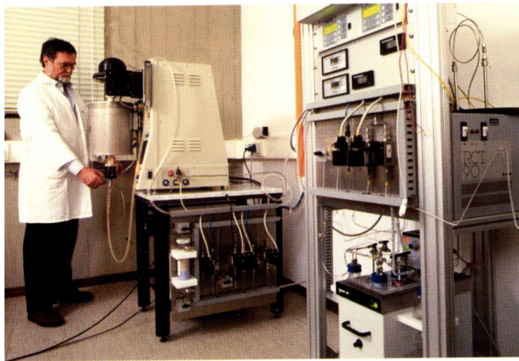
Facility for thermogravimetry with gas mixing and analysis station for high temperature corrosion testing up to 1700° C
