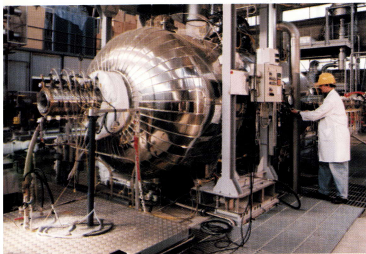
STORM: Investigation of aerosol behaviour in nuclear accidents and in industrial equipment
