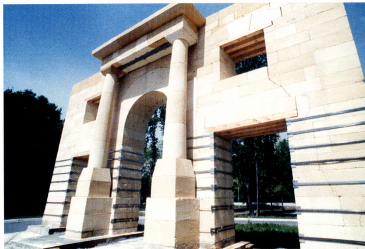
Earthquake behaviour of a historic monument investigated at the European Laboratory for Structural Assessment
