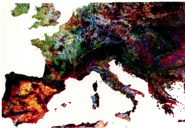
Color composite image derived from NOAA/AVHRR channel 1 and 2 data (year 1991). Red = annual minimum red reflectance. Green = annual maximum Near Infrared reflectance. Blue = annual Near Infrared reflectance standard deviation. This compositing is a first step toward the obtaining of a European land cover image.
