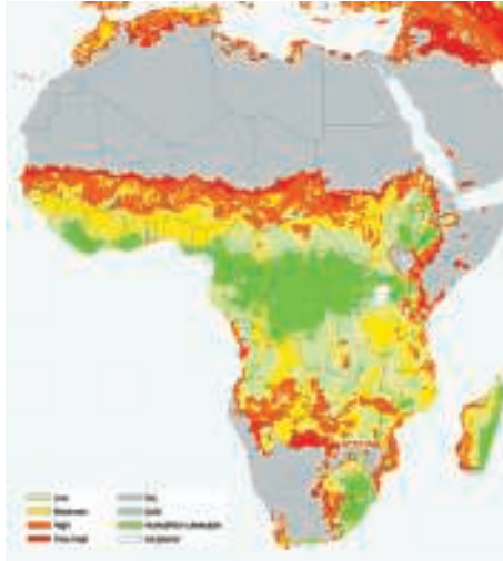
Map 4: Africa's environmental vulnerability.
