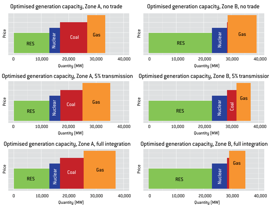
Figure 6: Energy support for Zones A and B, with optimisation and varying levels of trade
