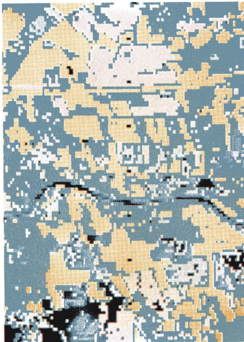
Fig. 14 - Supervised Fix-Hodge method
