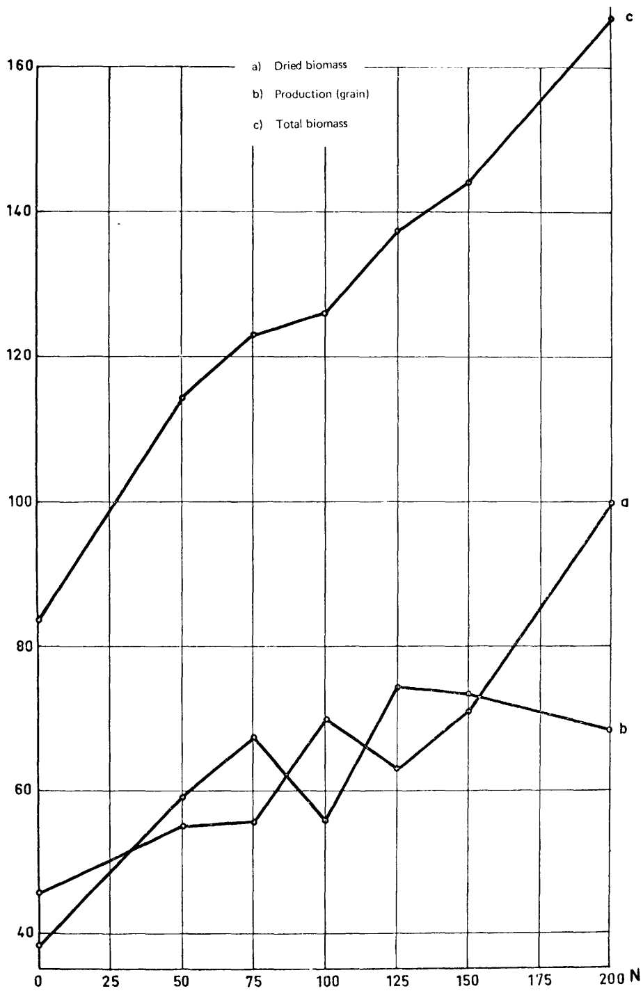
Fig. 41 - Biomass in relation to N-fertilization level
