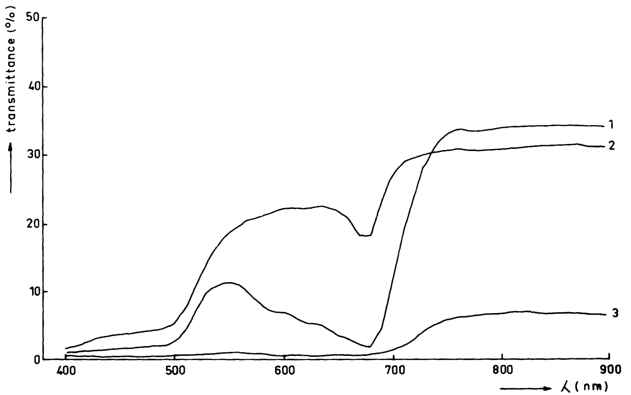
Fig. 78 - Transmittance of 1) green leaves, 2) yellow leaves, 3) stalk
