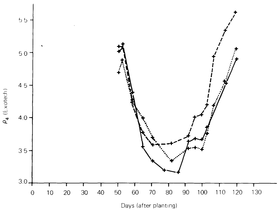
Fig. 68 - Evolution of visible light reflectance ( \rho_4 , Exotech) with time
