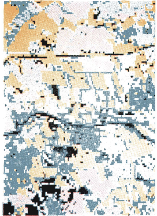
Fig. 13 - Supervised method, quadratic distance
