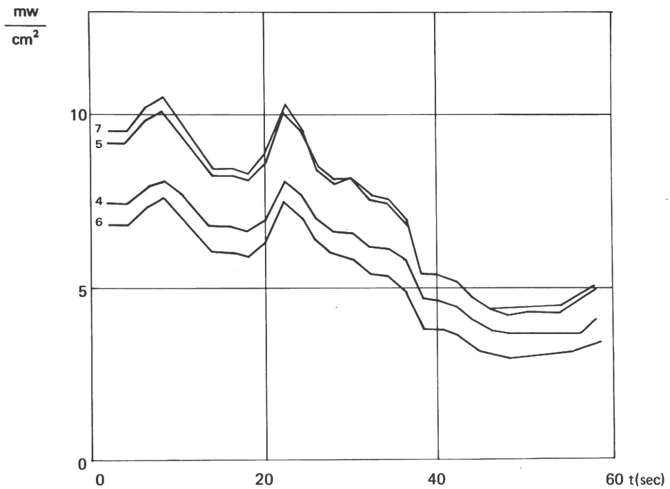
Fig. 120 - Incoming irradiance
