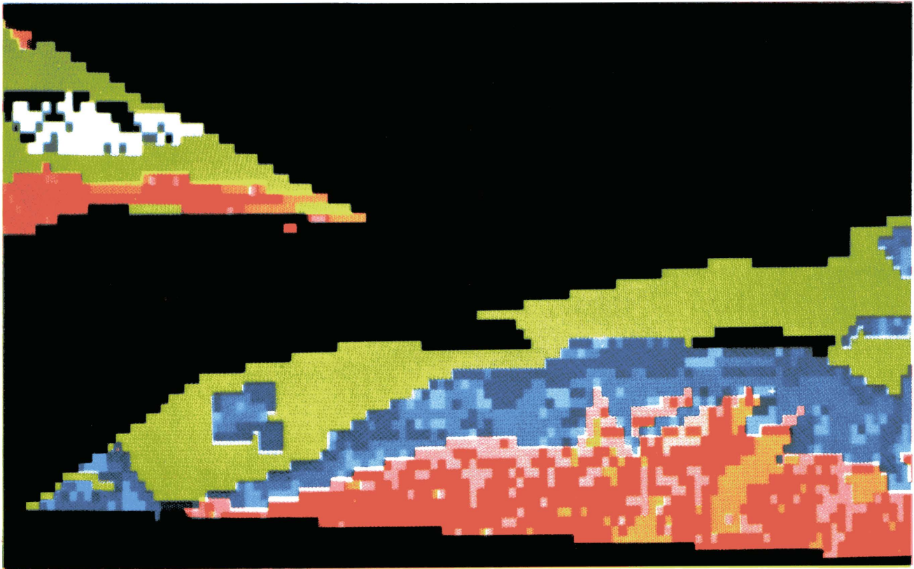
Fig. 108 - Display of performance matrix between ground truth and classification of Fig. 107 (ML method, 7/3/75 scene). Blue: chestnut recogn. as chestnut; light blue: chestnut classif. as beech; dark blue: other chestnut; red: beech recogn. as beech; purple: beech classif. as chestnut; orange/red: other beech; white: mixed deciduous forest classif. as beech; dark green: mixed deciduous forest classif. as chestnut; yellow/light green: crops and meadows (in any classification)
