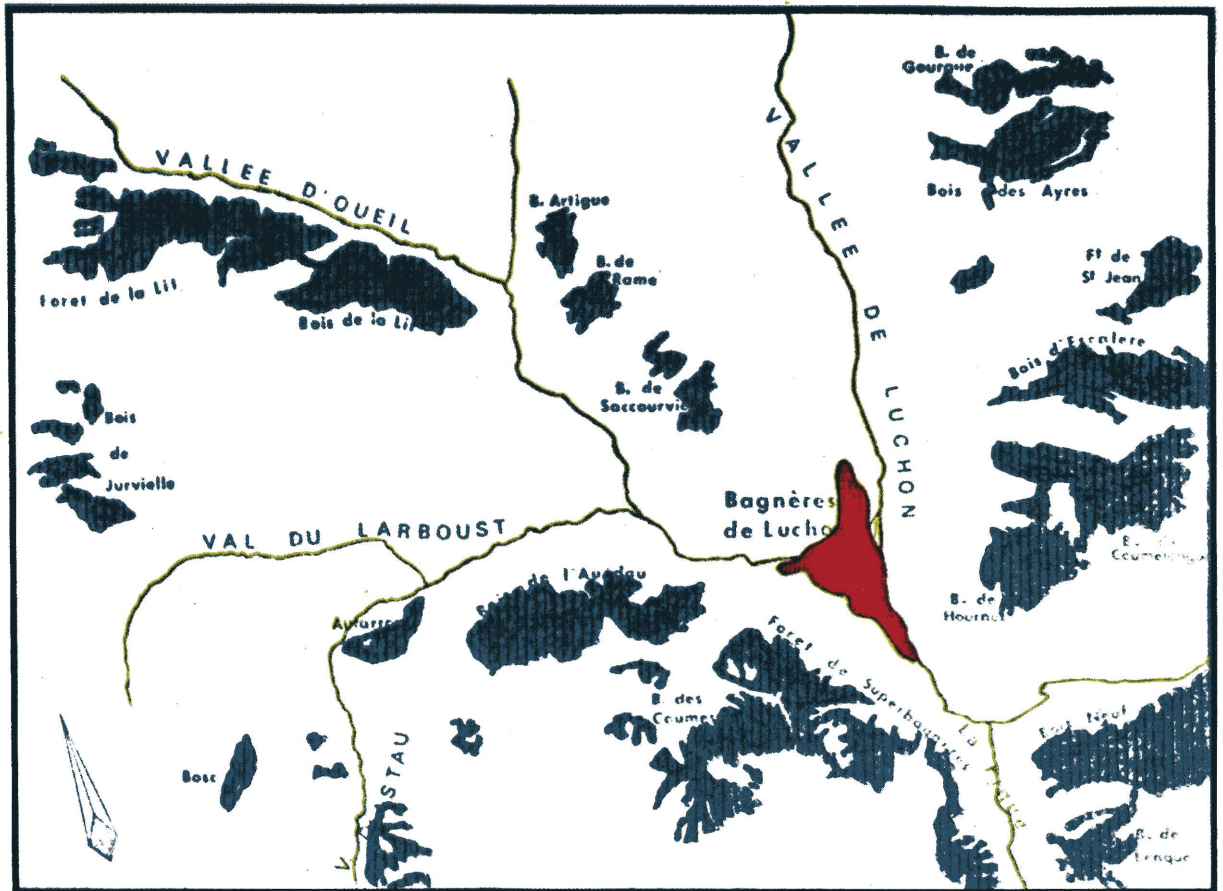
Fig. 110 - Reference map of fir forests from photointerpretation and ground data
