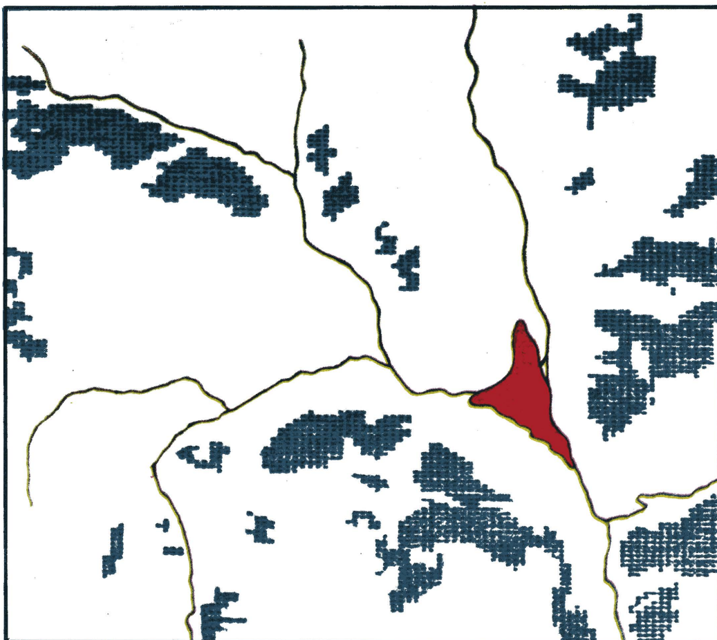
Fig. 111 - Digitized map of fir forests
