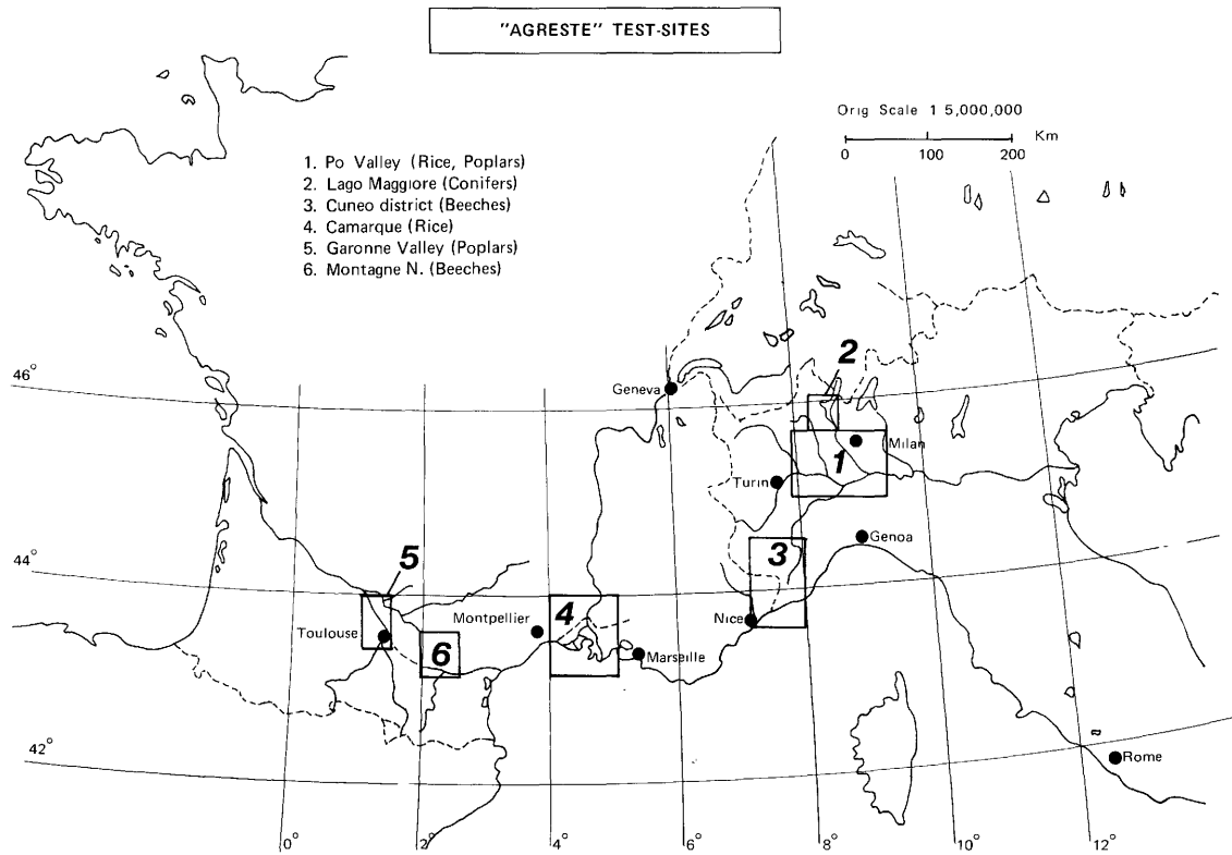
Fig. 1 - Geographic location of the European test sites in Southern France and Northern Italy
