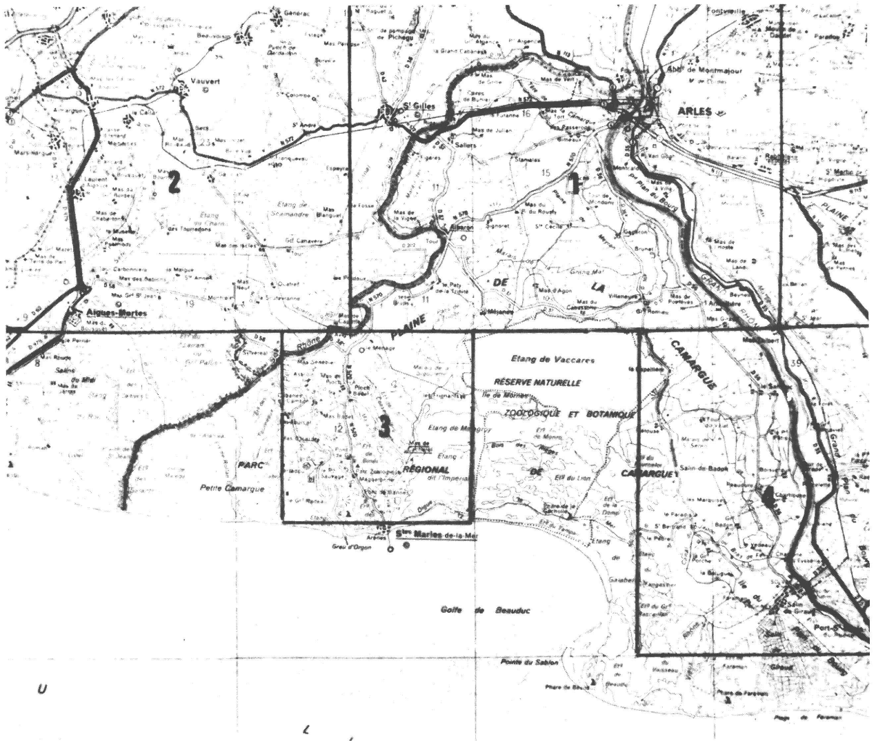
Fig. 4 - French test site No. 4 (about 55 x 20 km)
