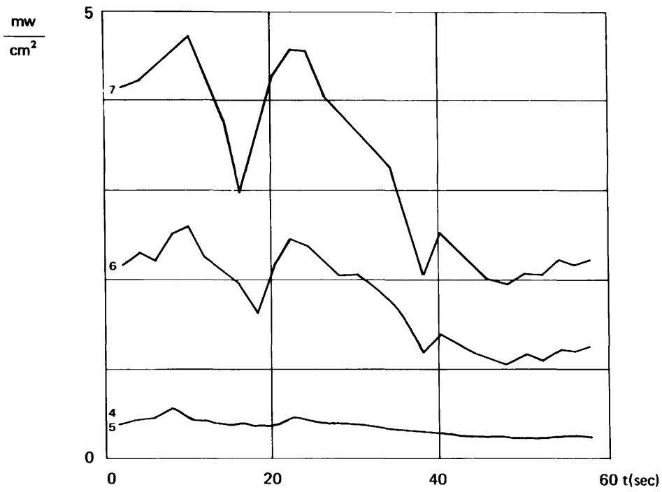
Fig. 121 - Reflected irradiance ( Salix alba )
