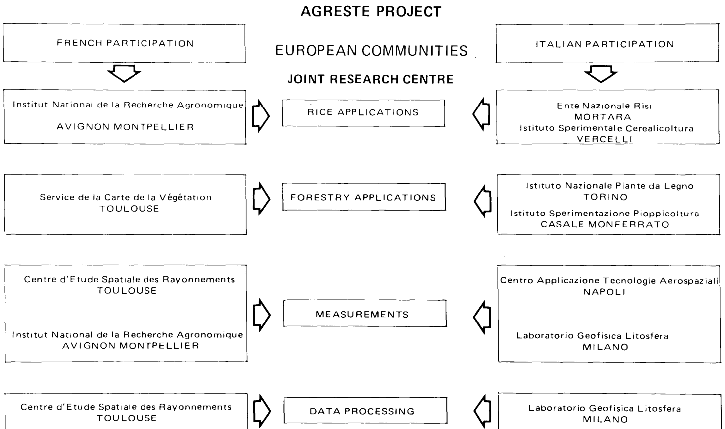
Fig. 2 - Participation in the AGRESTE Project
