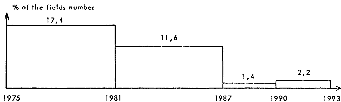
Fig. 93 - Forecast of Robusta available timber
