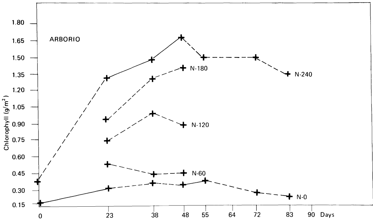
Fig. 27 - Evolution of chlorophyll index with time
