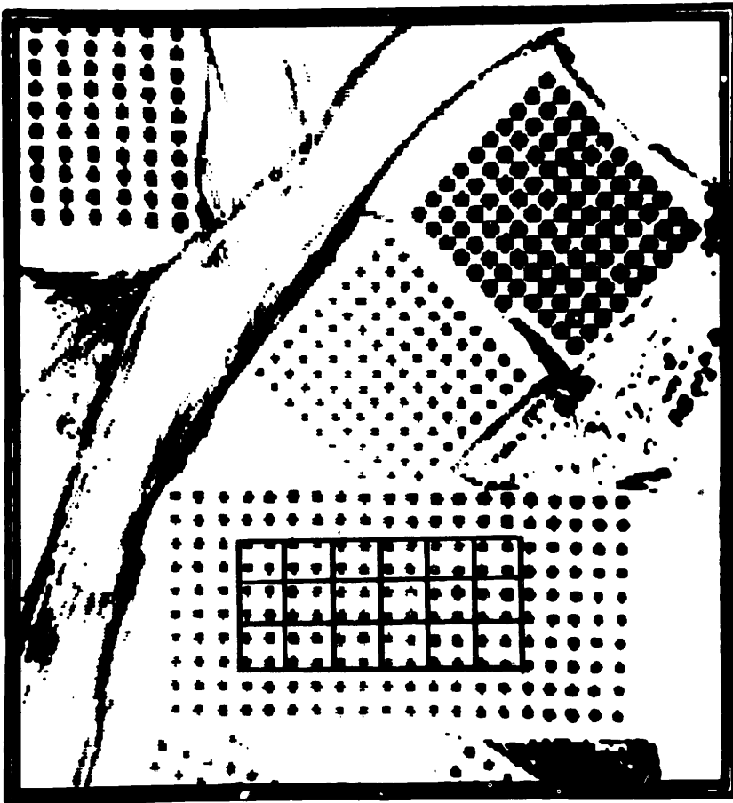
Fig. 96 - Display of some simulated plots
