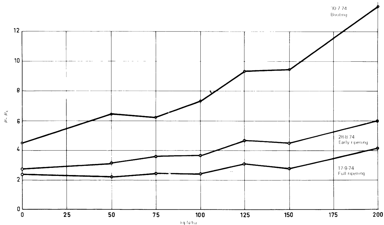
Fig. 43 - Reflectance ratio in relation to N-fertilization level
