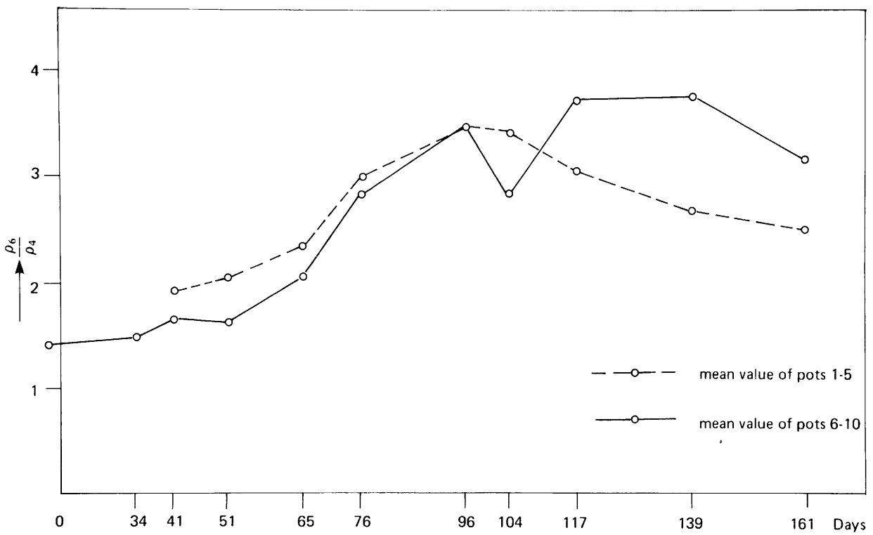
Fig. 26 - Evolution of ratio \rho_6/\rho_4 with time
