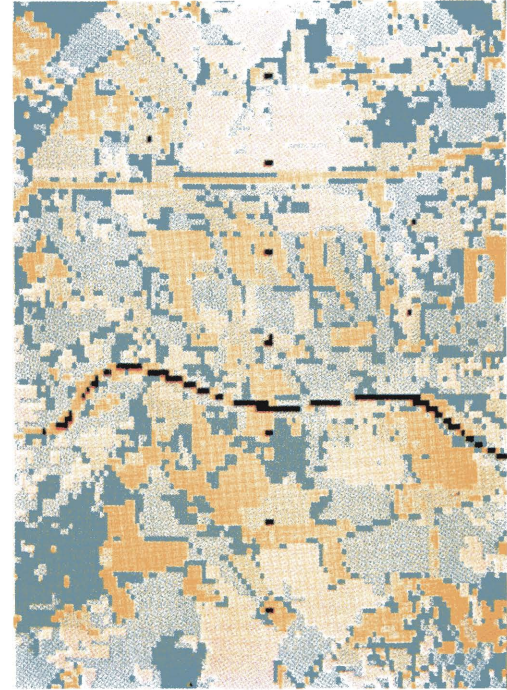
Fig. 15 - Unsupervised method, Mahalanobis distance
