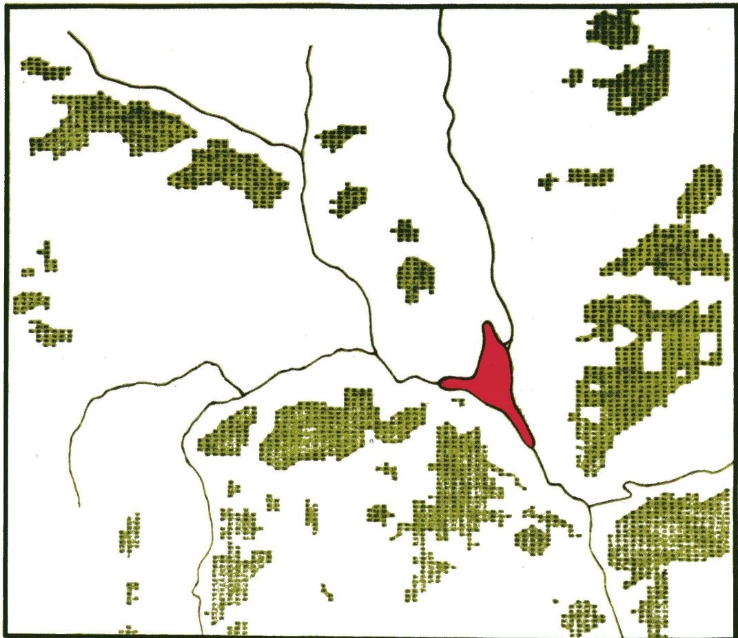
Fig. 116 - Results of the preceding fig. after smoothing
