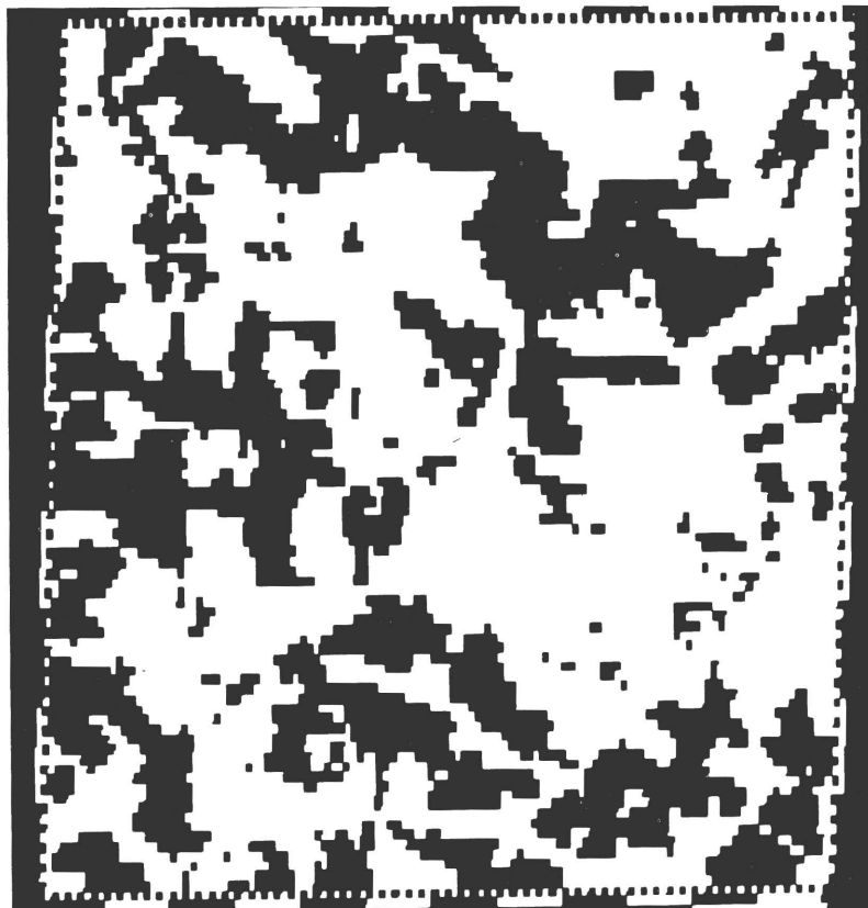
Fig. 20 - Map of classified rice fields (in black) obtained by level slicing of LANDSAT channel 7 on May 10, 1973, test area "Ferrera"
