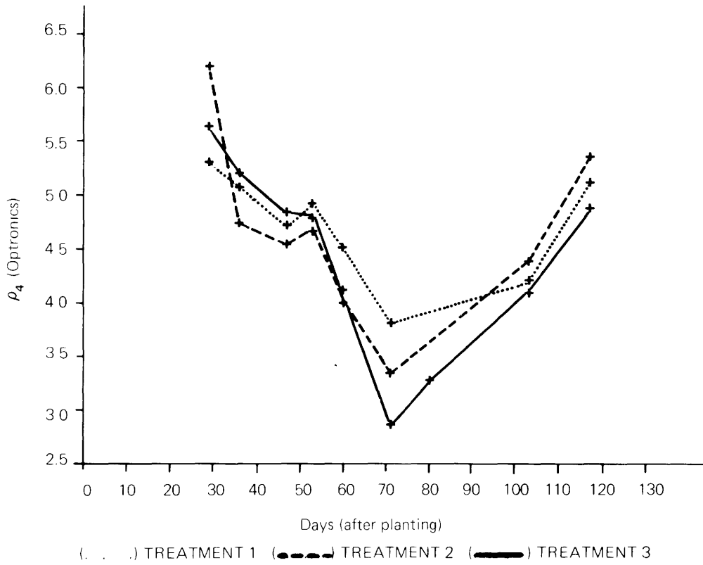
Fig. 67 - Evolution of visible light reflectance ( \rho_4 , Optronics) with time
