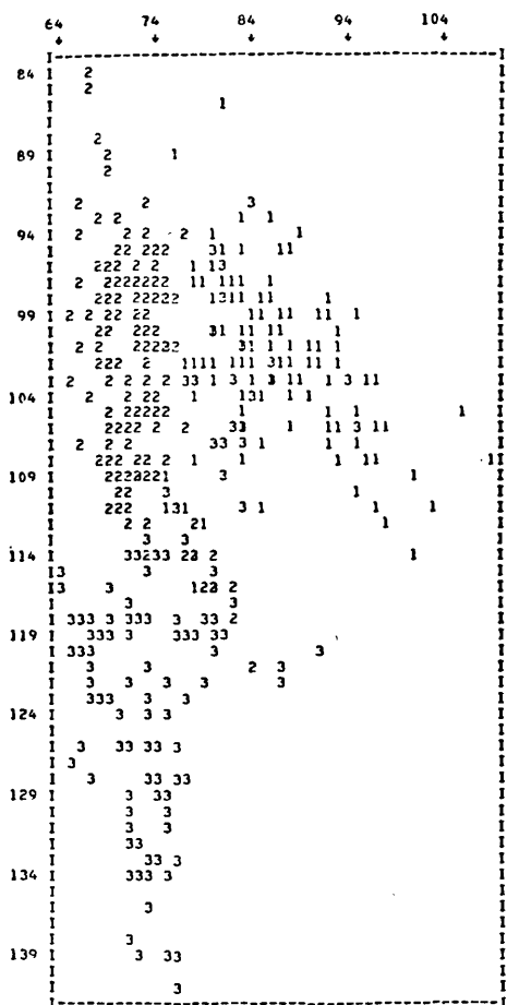
Fig. 9 - Bispectral diagram of the responses of samples on MSS 5 and MSS 7 channels (1: rice fields; 2: vineyards; 3: cereals)
