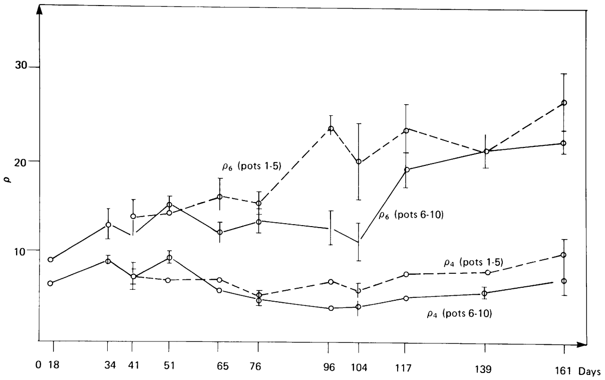
Fig. 25 - Evolution of reflectance \rho_4 and \rho_6 with time
