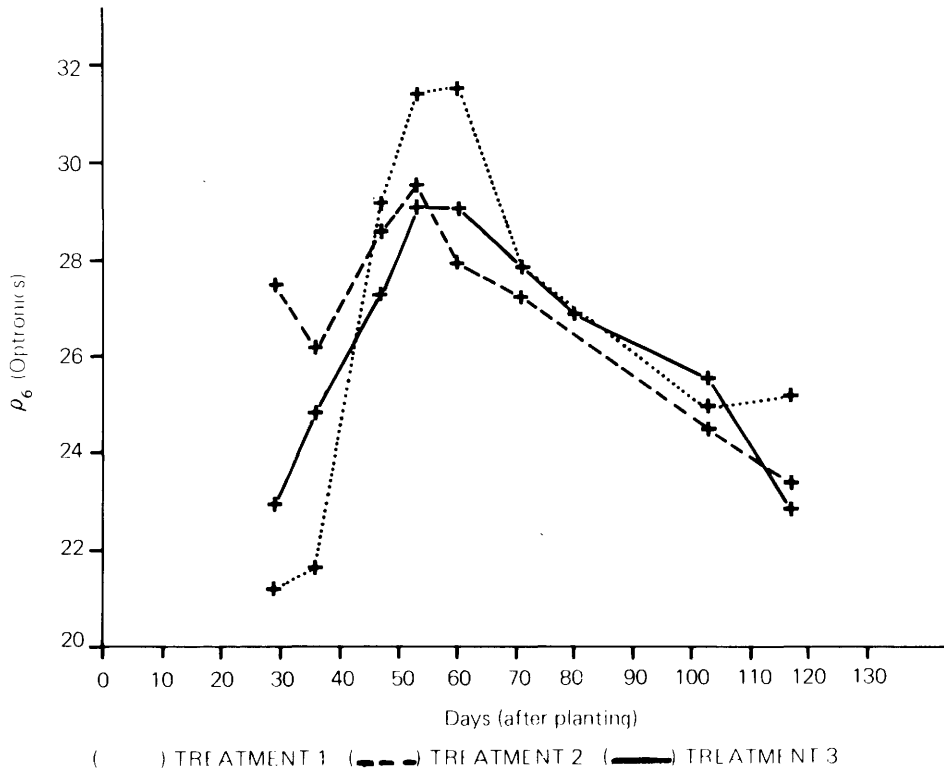
Fig. 64 - Evolution of near infrared reflectance (Optronics) with time
