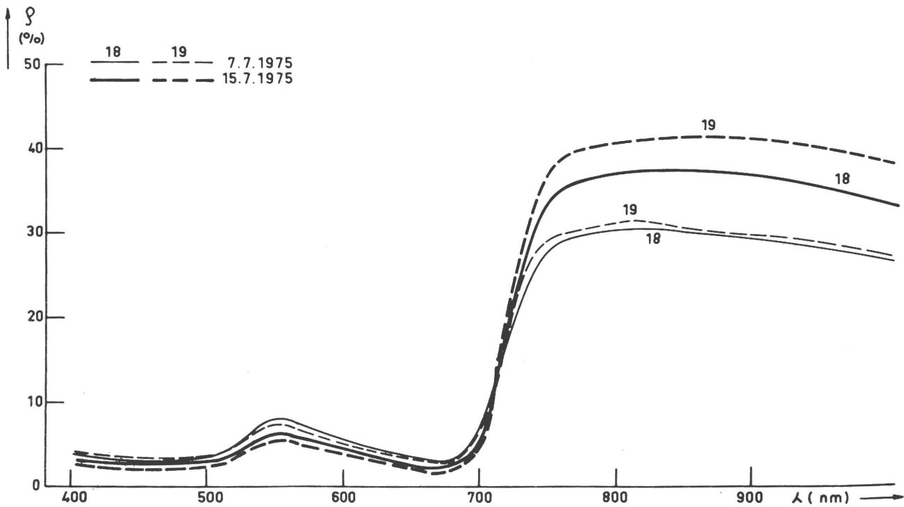
Fig. 76 - Measured spectral reflectance of rice lysimeters No. 18 and 19
