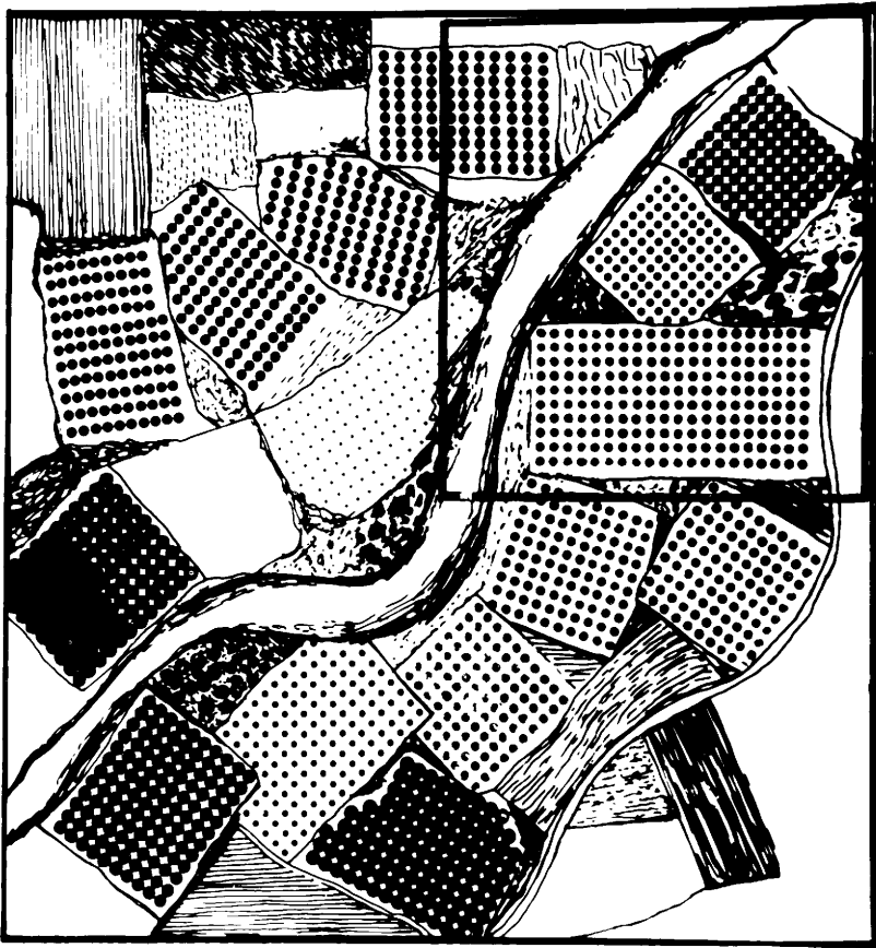
Fig. 95 - Theoretical model of poplar coverage
