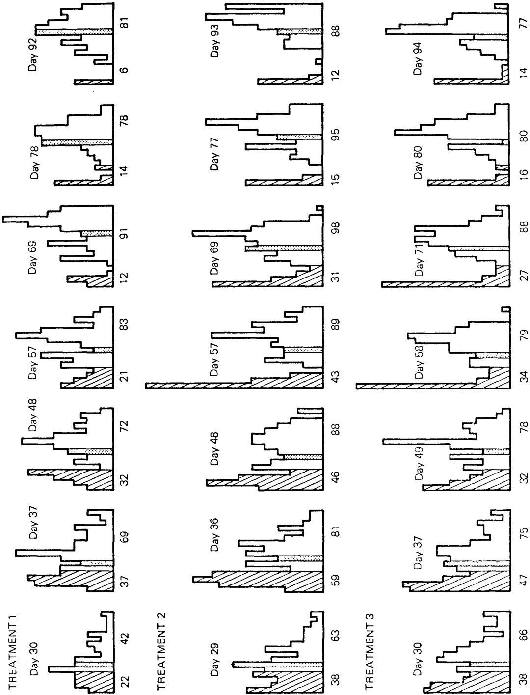
Fig. 62 - Frequency distribution of halm weights in 7 successive samplings on 5 x 4 plants
