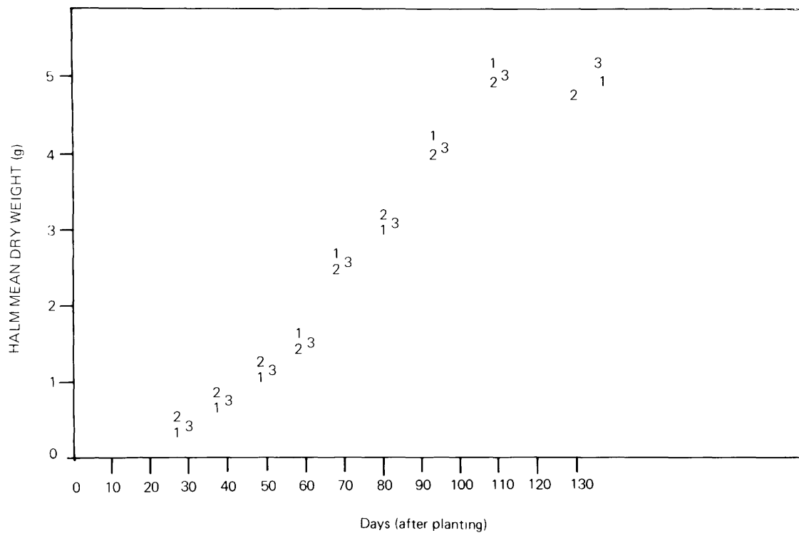
Fig. 58 - Halm growth in the three treatments
