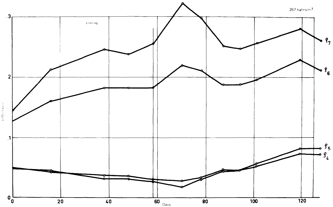
Fig. 53 - Evolution of reflectances with time, at density 287 halms/m 2
