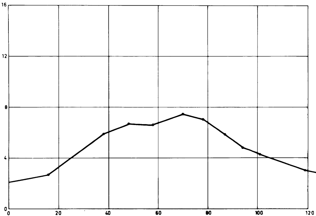
Fig. 55 - Evolution of reflectance ratio \rho_7 / \rho_5 with time, density 212 halms/m 2
