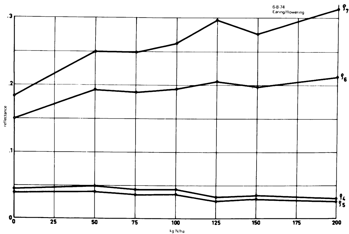
Fig. 42 - Reflectances in relation to N-fertilization level
