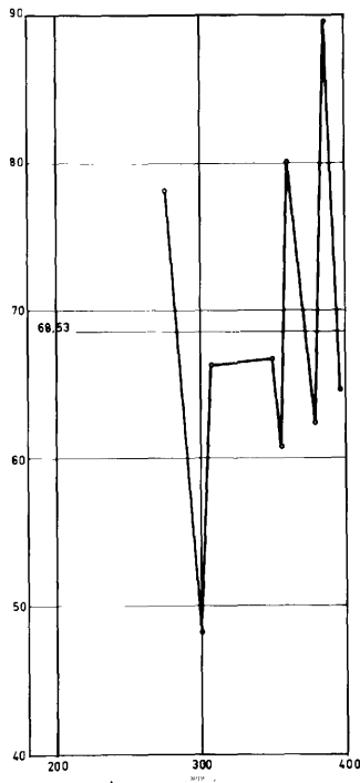
Fig. 48 - Grain production in relation to density, in normal density field conditions
