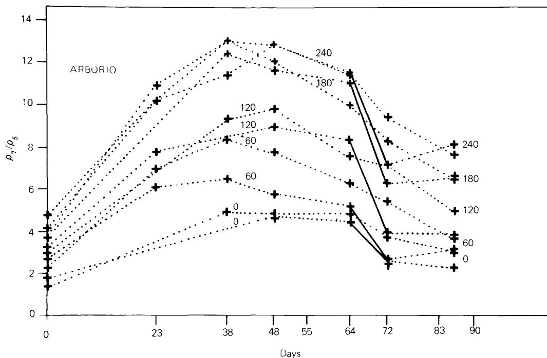
Fig. 36 - Evolution of reflectance ratio \rho_7/\rho_5 with time
