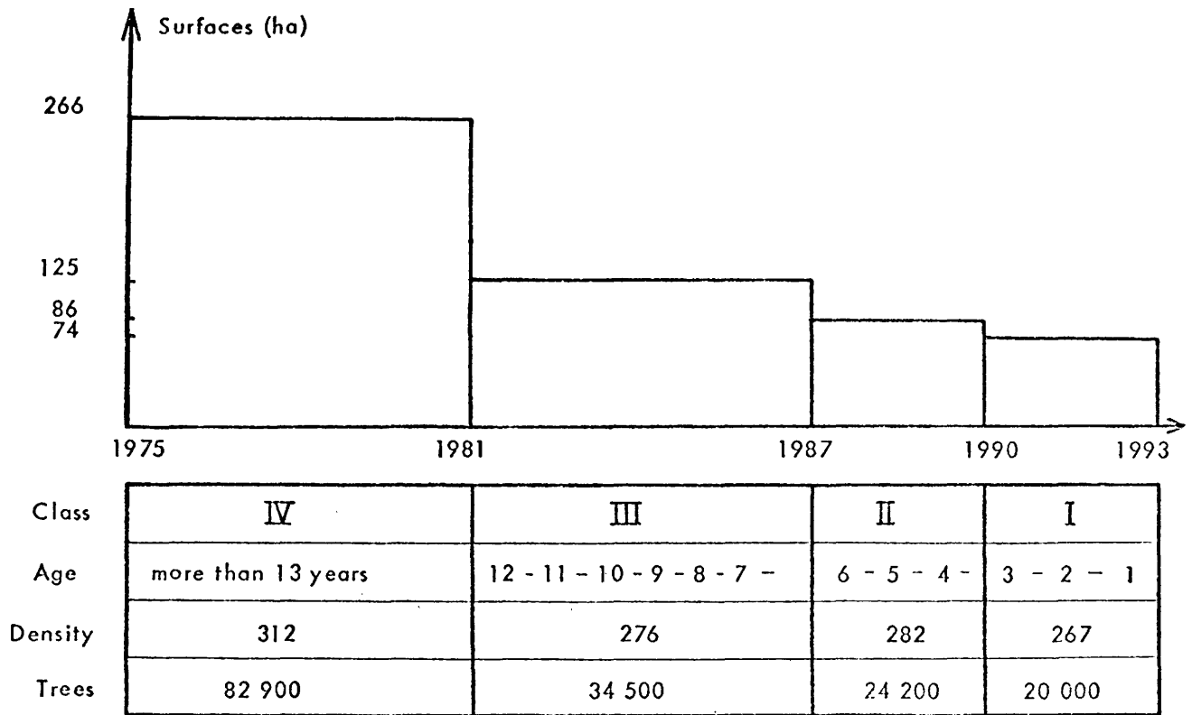
Fig. 90 - Global forecast of available timber
