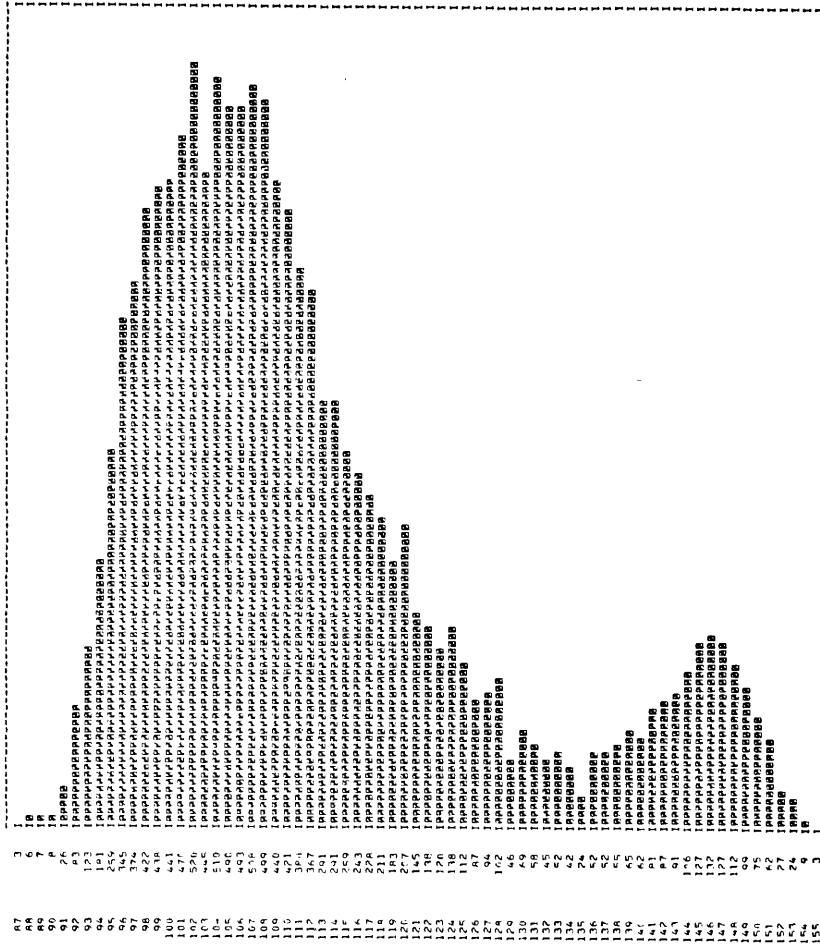
Fig. 102 - Histogram of cover rate of poplar grove no. 4 (of Fig. 101)
