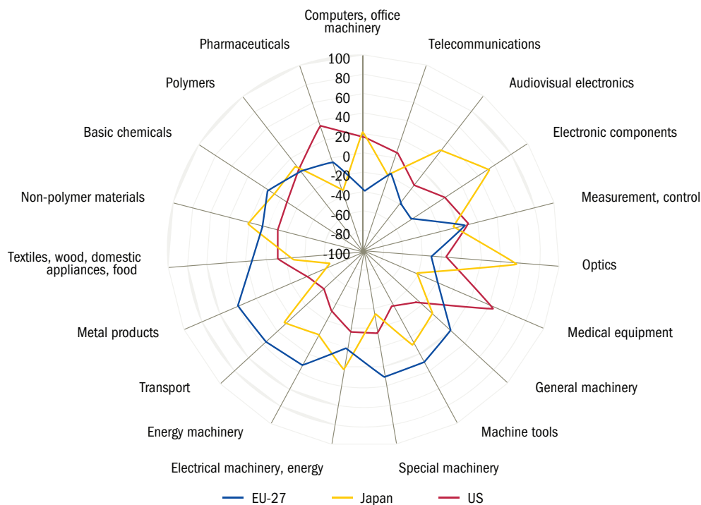
FIGURE I.3.6 Technology specialisations (2004-2005)
