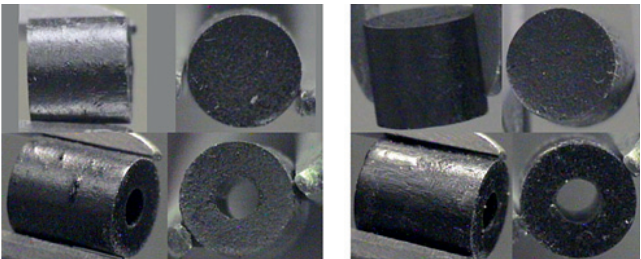
Figure 44 - HELIOS fuel pellets of pin 3, (Zr, Y, Am, Pu) \text{O}_2 (Note: Pin 3 is instrumented with a Thermocouple then contains annular pellets)
