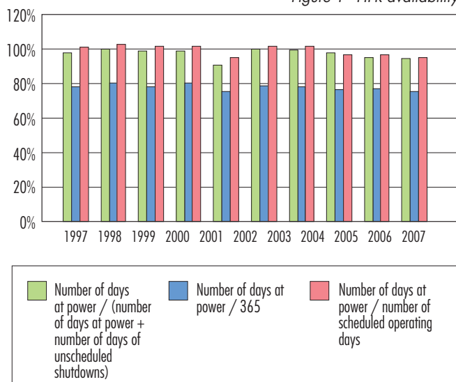
Figure 1 - HFR availability
