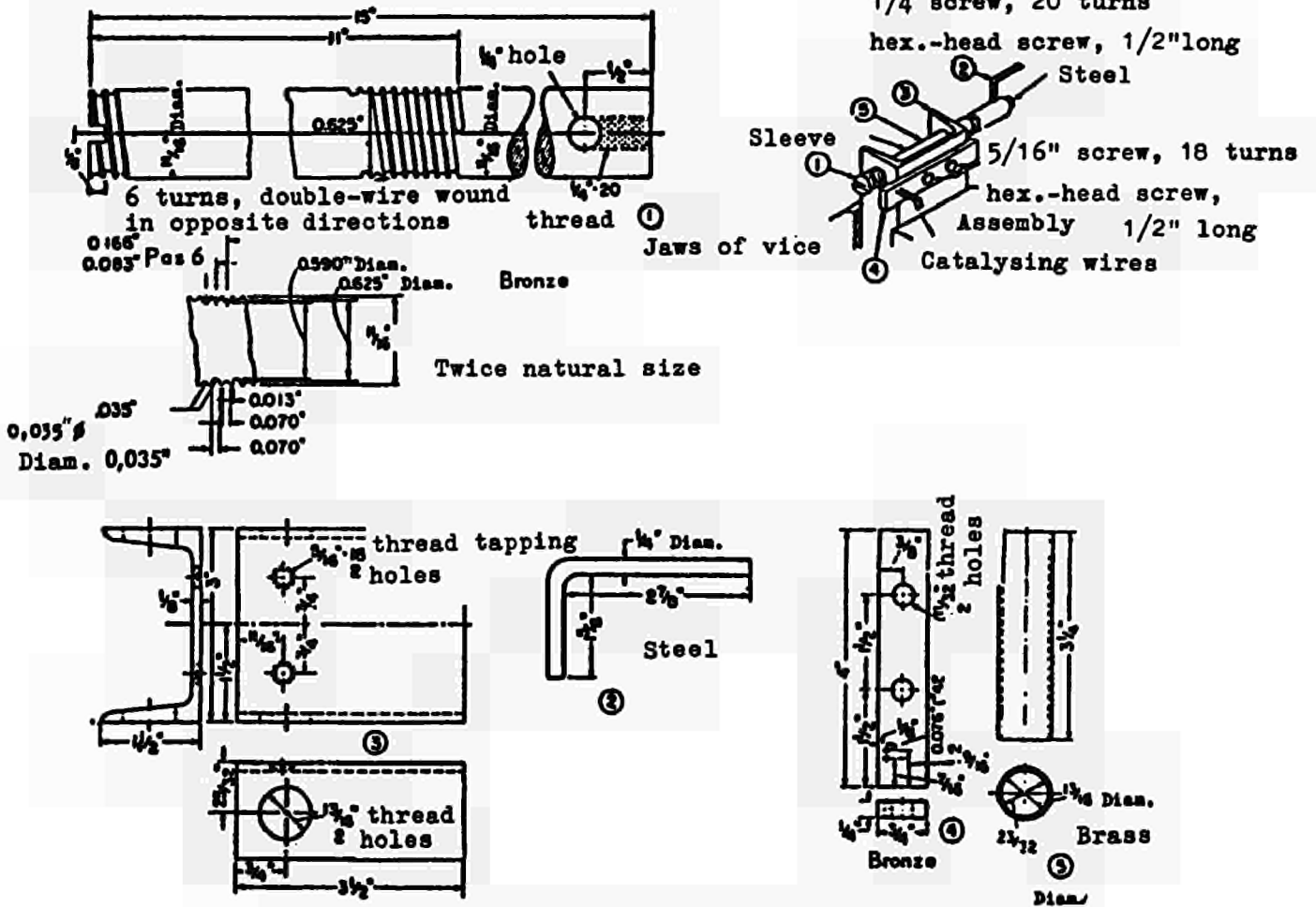
Fig. 2: SPINDLE FOR WINDING CATALYZING COILS
