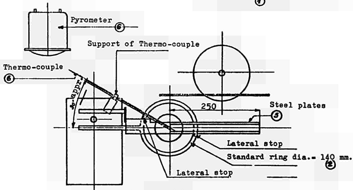
Details of Thermo-couple supports and lateral stops
