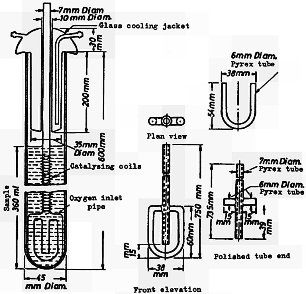
Fig. 1: OXIDIZING CELL
