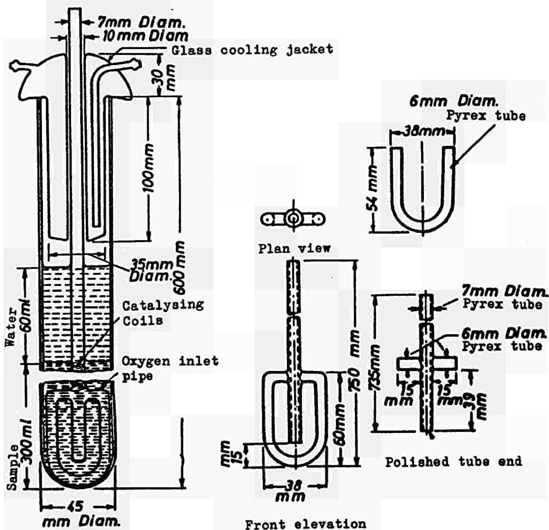
Fig. 1: OXIDIZING CELL
