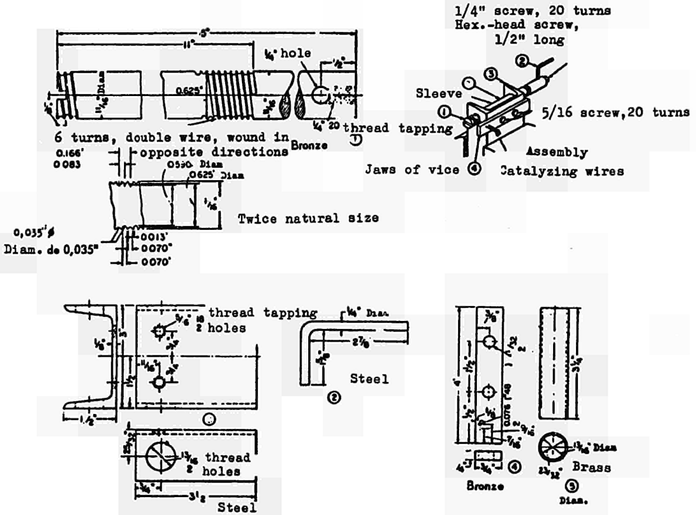
Fig. 2: SPINDLE FOR WINDING CATALYZING COILS
