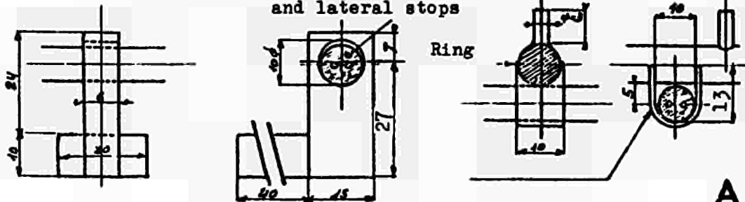
Details of Thermo-couple supports and lateral stops
