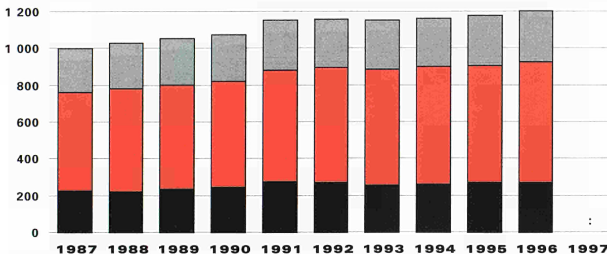
Energy transformed (input) by power stations and refineries, million toe. EU-15
