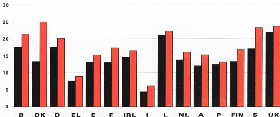
Electricity prices for small standard consumers: 600 kWh per year, ECU per 100 kWh. 1 July 1997
