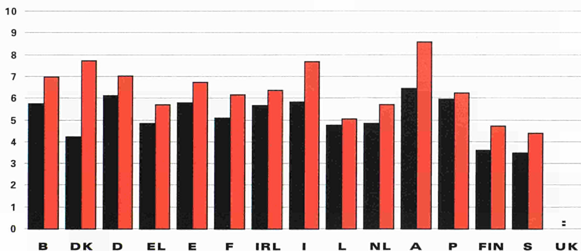
Electricity prices for large industrial standard consumers: 24 GWh per year, ECU per 100 kWh. 1 July 1997
