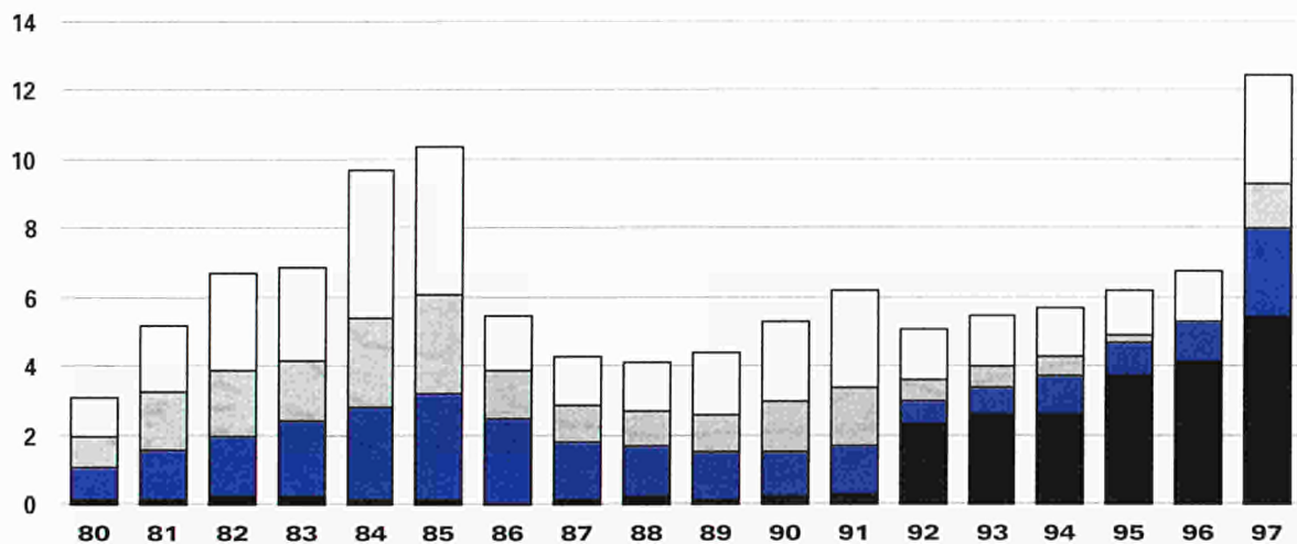
Extra-EU imports of natural and manufactured gas by main providers. 1000 million ECU
