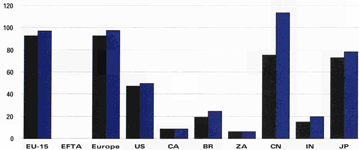
World production of pig iron. Million t. 1992 and 1997
