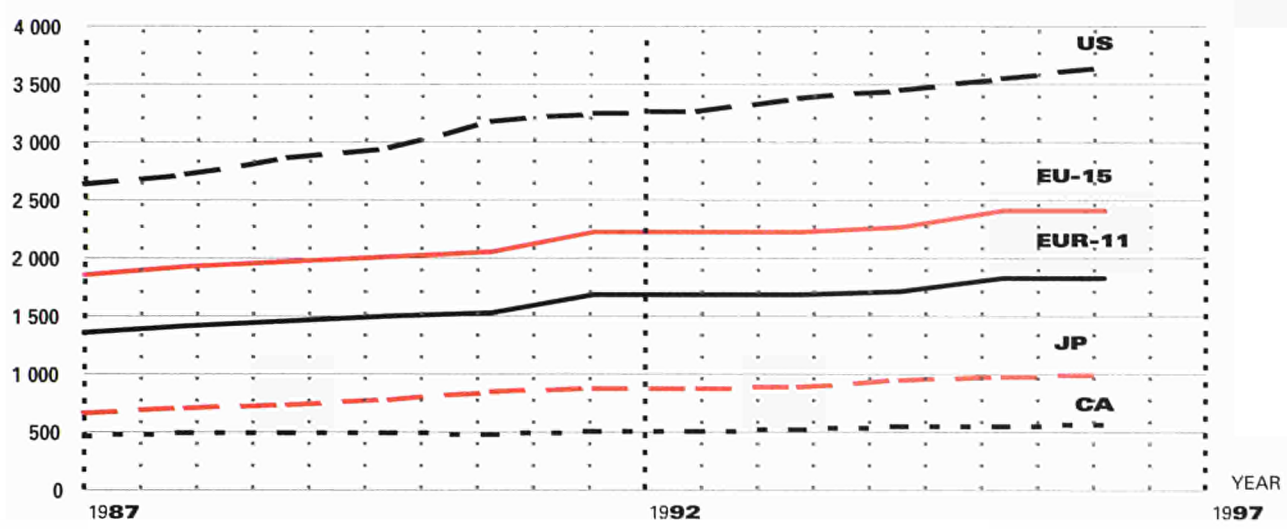
Electricity production, 1000 GWh 3B5DG
