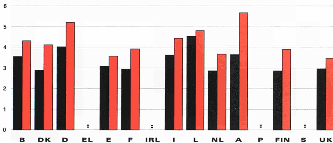
Natural gas prices for large industrial standard consumers: 418 600 GJ per year, ECU per GJ. 1 July 1997
