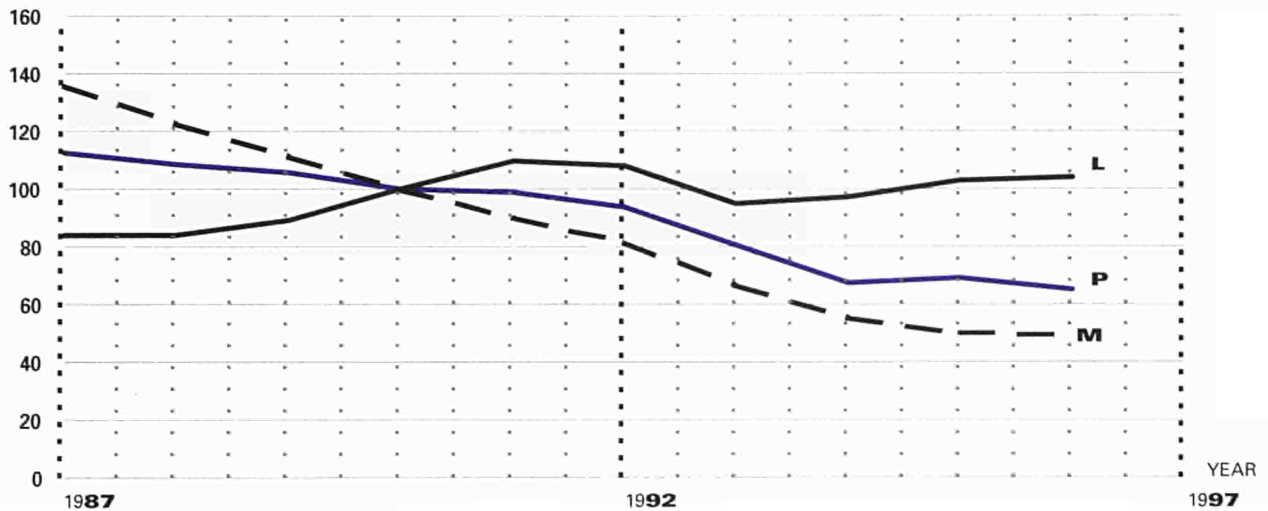
Hard coal industry: production, imports and underground employment. 1990 = 100. EU-15
