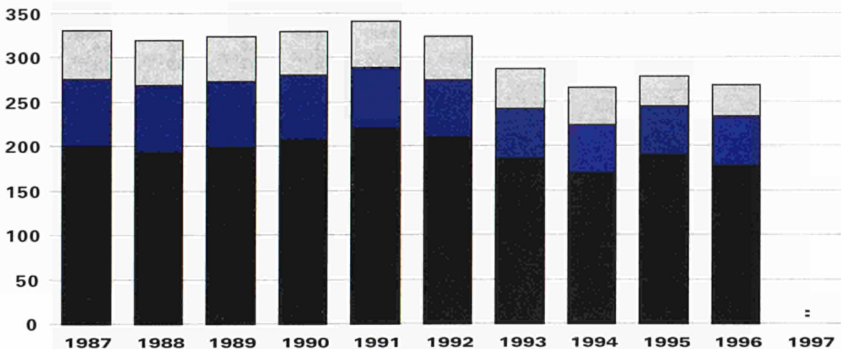
Hard-coal deliveries to major consumers: public and pithead power stations coking plants and other consumers. Million t. EU-15
