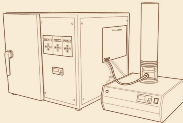
The operating principle of the prototype chemiluminometer which should enable librarians to assess paper degradation.
