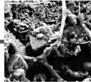
Detailed microphoto of the marble structure covered in black dust – Freedom Monument, Riga (LT).
